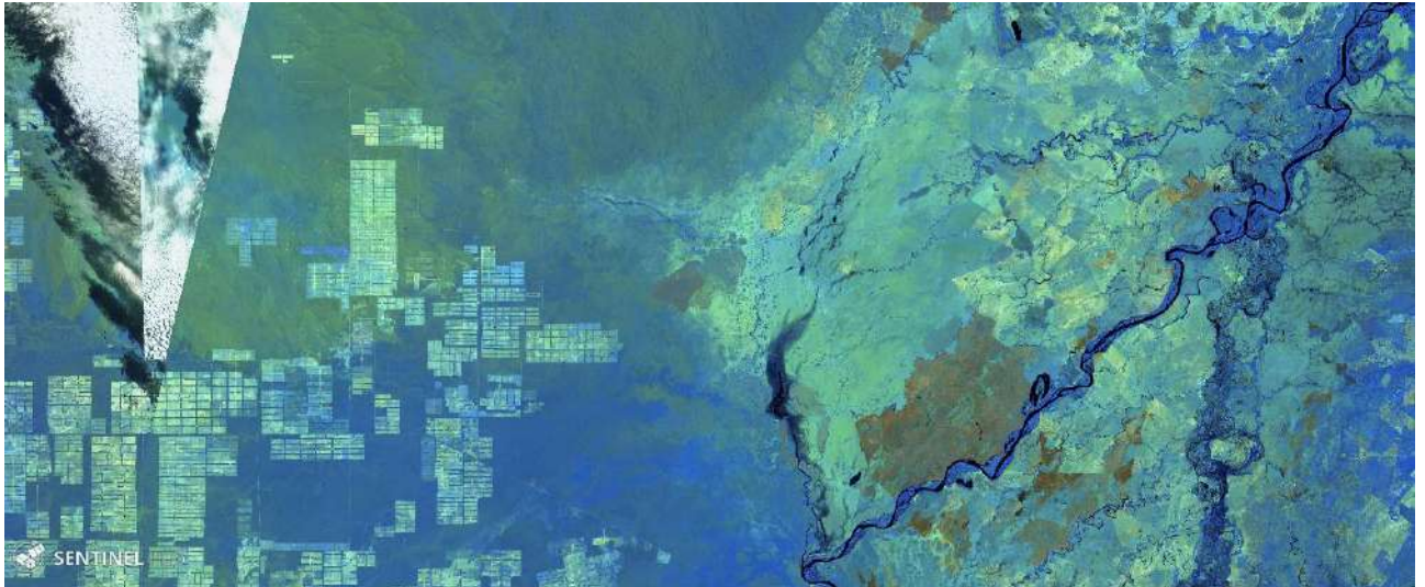
Figura 7 - Corumbà, Mato Grosso do Sul (Brazil). 05.08.2019. Pre - fire image - atmospheric penetration visualization
