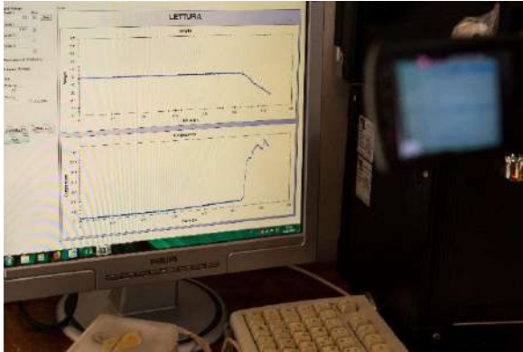
Figure 2 - Combustion chamber analysis at IRET CNR
