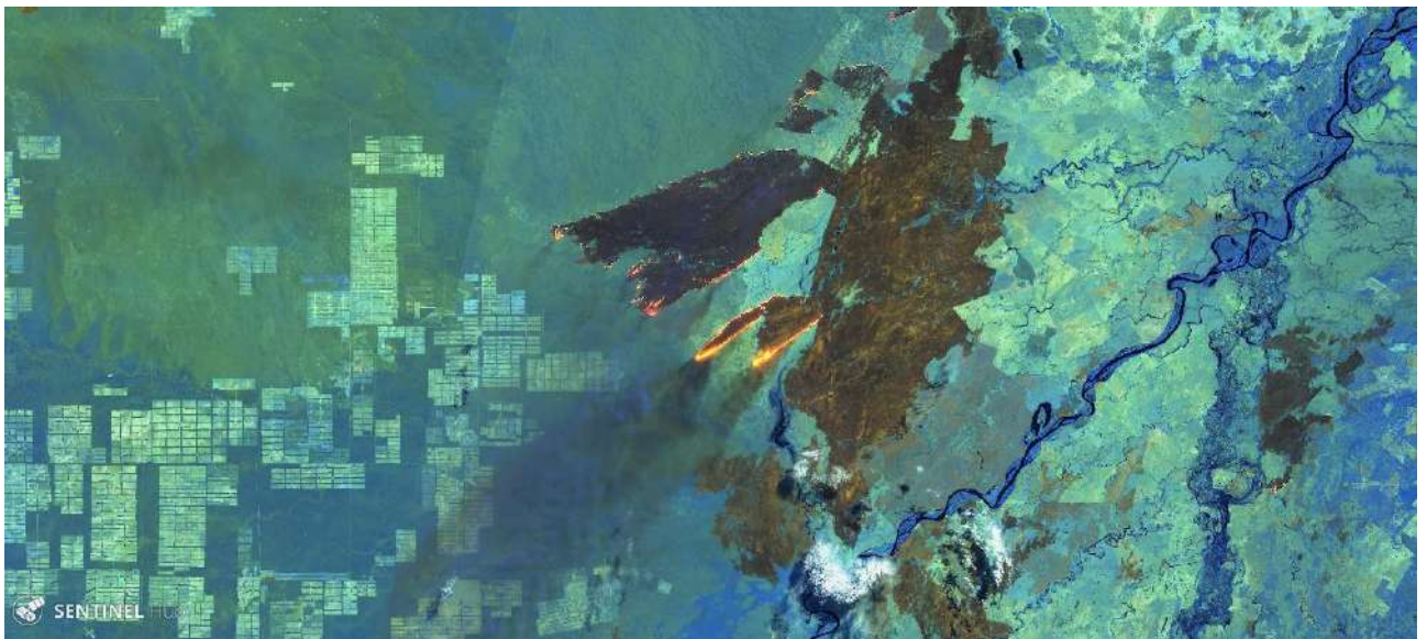
Figure 8 - Corumbà, Mato Grosso do Sul (Brazil). 28.08.2019. Post - fire image - atmospheric penetration visualization
